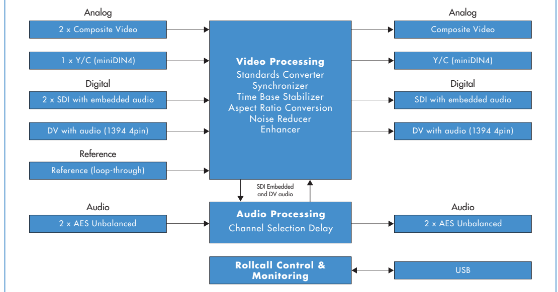
CVR600UDV SDI, DV & Composite Standards Converter
