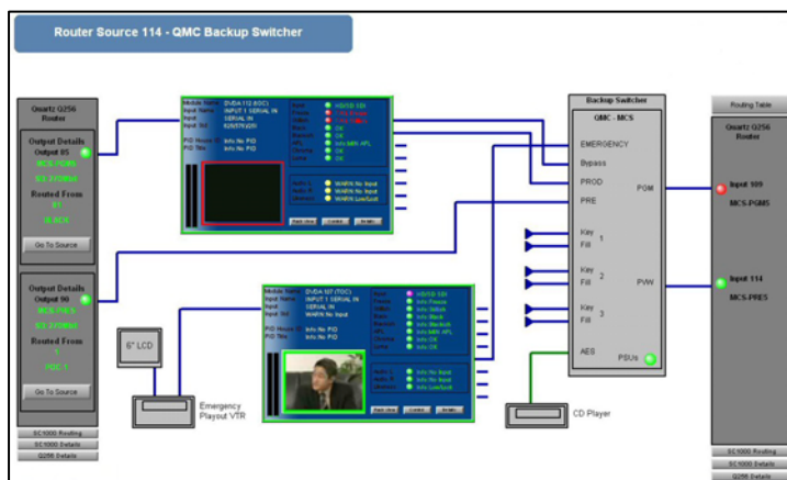
Example of single signal path monitoring with 3rd party router and switcher monitoring including dynamic tallies and display of routing dynamically
